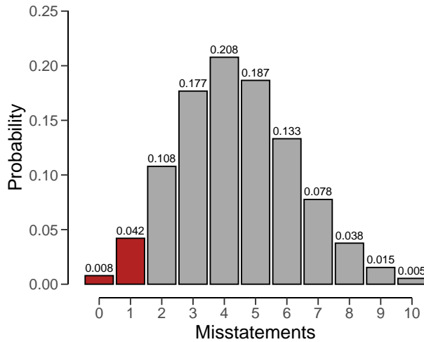
Figure 4.3. The \text{hypergeometric}(k \mid 147, 1000, 30) distribution showing the probability for k = 0 and k = 1 misstatements as a red bar.
