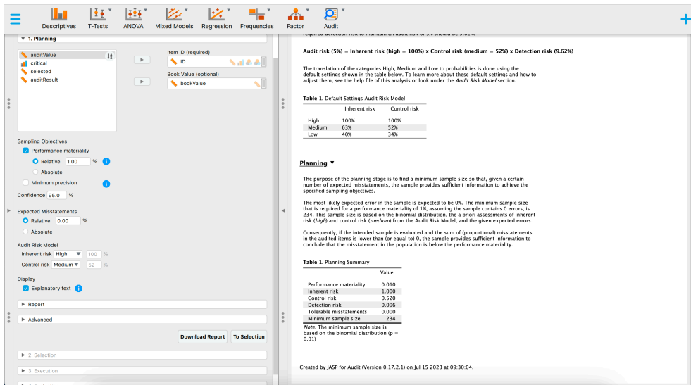
Figure 8.10. A snapshot of the planning stage for this example in the sampling workflow analysis in JASP for Audit.
