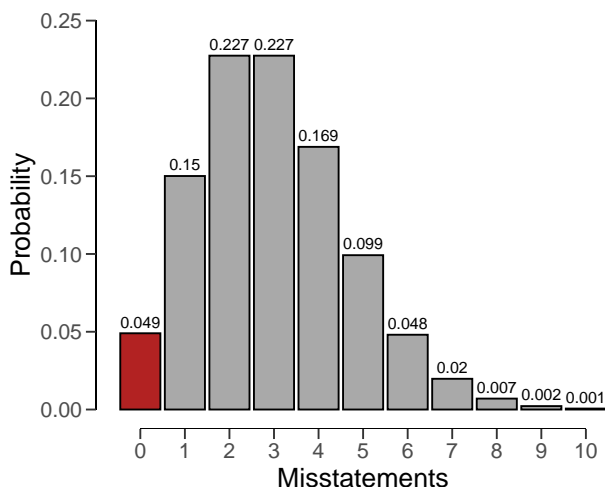
Figure 4.6. The \text{binomial}(k \mid 99, 0.03) distribution showing the probability for k = 0 misstatement as a red bar.
