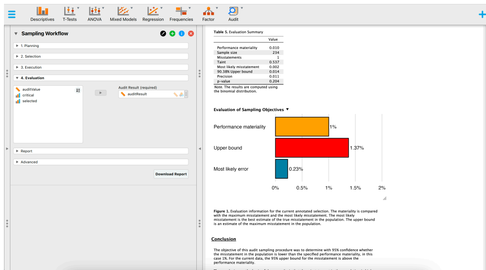
Figure 8.12. A snapshot of the evaluation stage for this example in the sampling workflow analysis in JASP for Audit.
